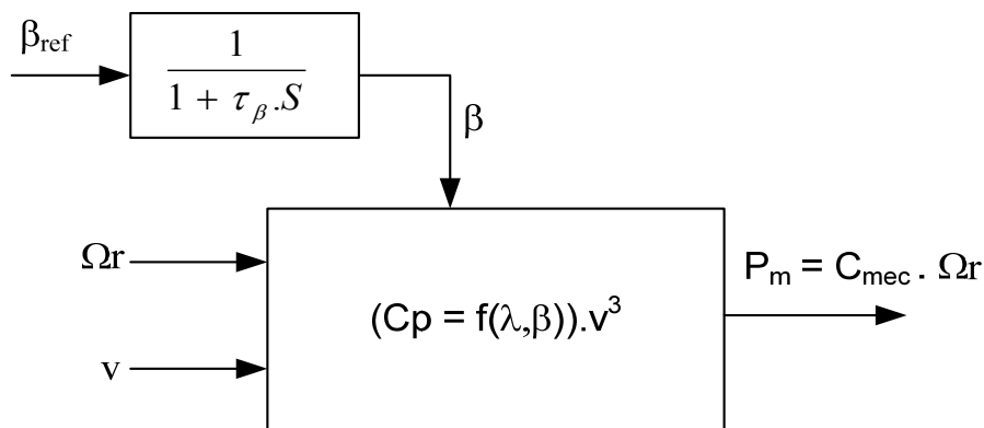
Figure 2. Schematic of a wind turbine
