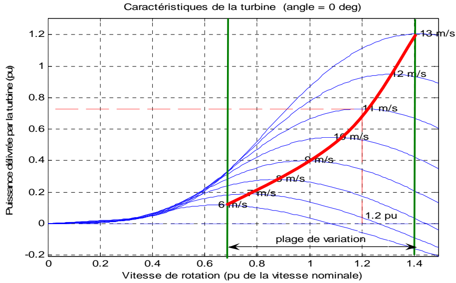
Figure 3. Turbine characteristics
