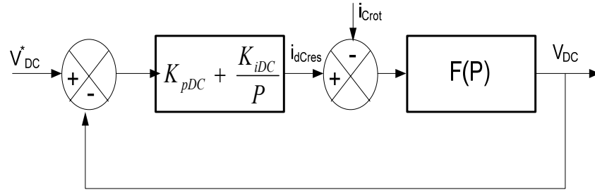
Figure 6. Continuous bus voltage Regulation block diagram
