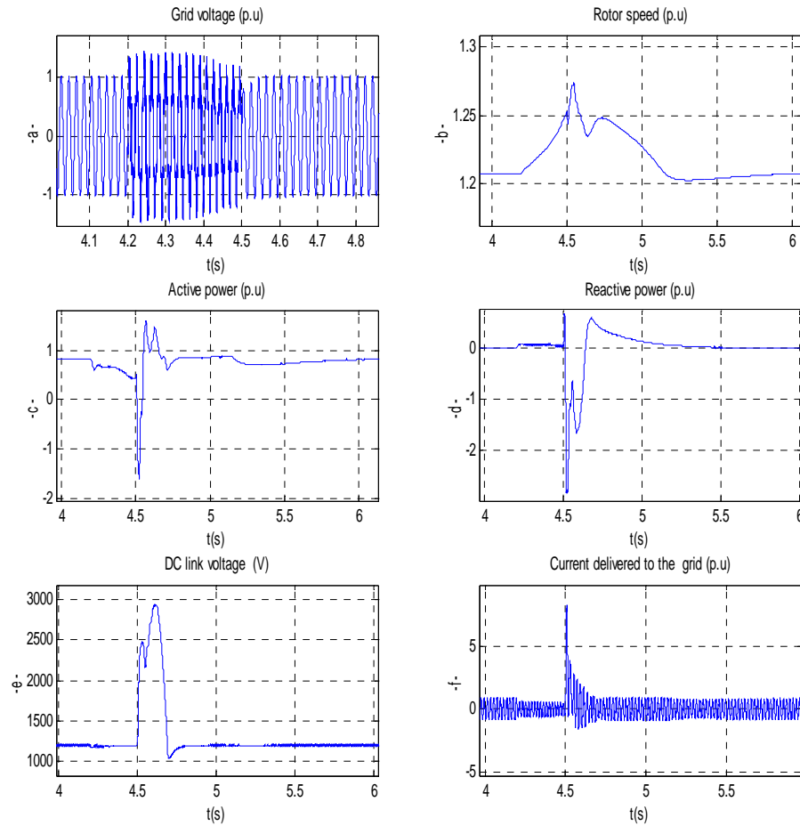
Figure 12 Results obtained with a PI regulator a- Grid voltage, b- Generator speed, c- Active power, d- reactive power, e- DC link voltage, f- Rotor active power
