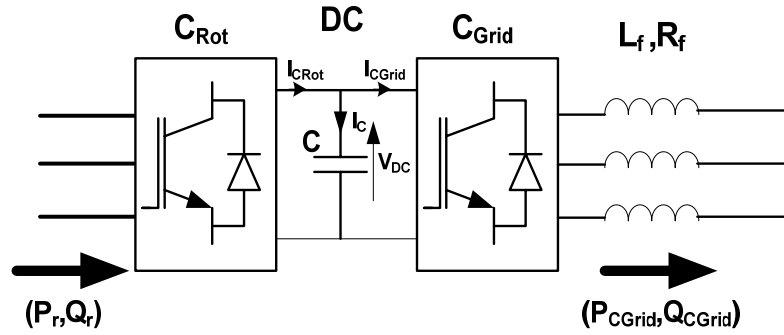
Figure 4. Unified Power Flow Controllers (UPFC)
