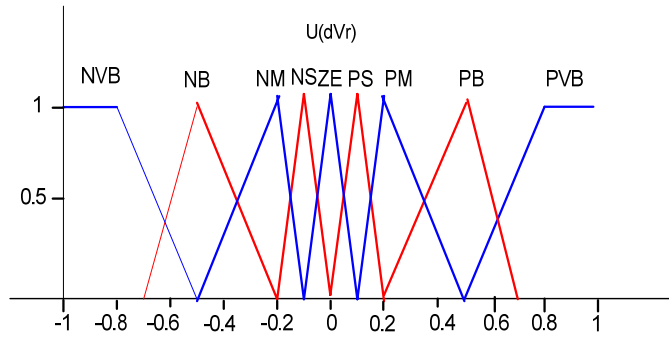
Figure 15. Output membership functions.
