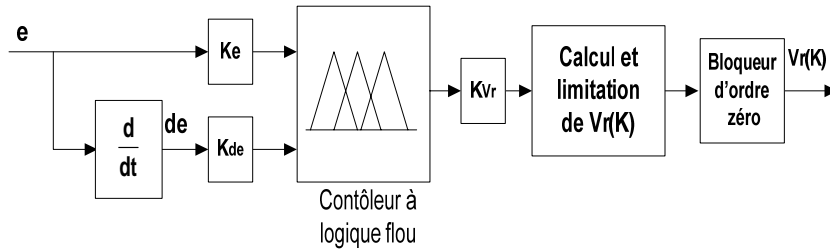
Figure 13. Diagram of fuzzy logic controller.
