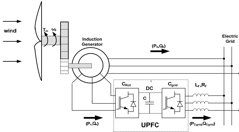
Figure 1. Configuration of a Doubly Fed Induction Generator (DFIG).
