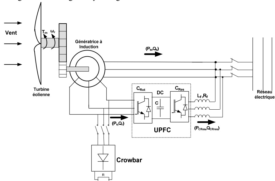
Figure 10. Diagram of A Wind Turbine Based On DFIG Using A Crow-Bar System.
