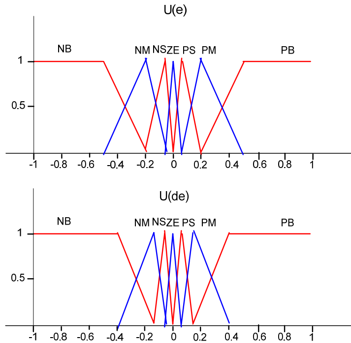
Figure 14. Inputs membership functions
