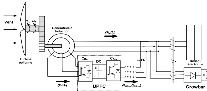
Figure 11. Doubly Fed Induction Generator (DFIG) with a crowbar system.
