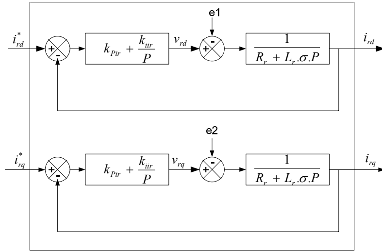
Figure 5. Rotor current regulator diagram block
