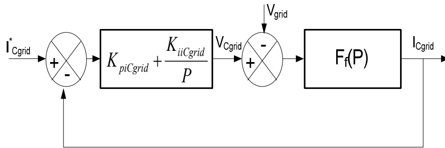
Figure 7. Cgrid Converter current Regulation block diagram
