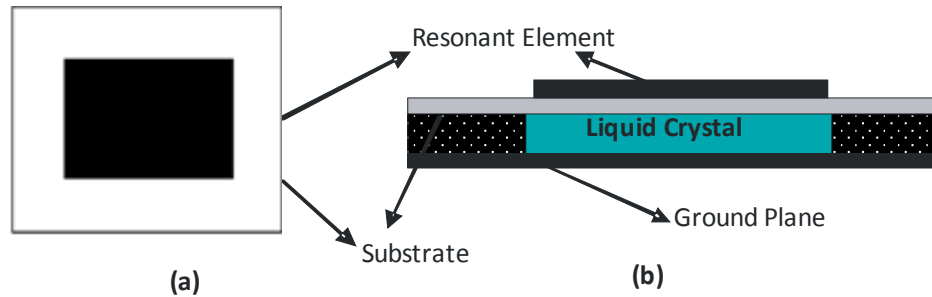
Figure 2. Built configuration of a unit cell reflectarray element (a) Top View (b) Side view
