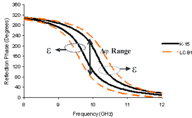
Figure 3. Dynamic phase ranges of anisotropic liquid crystal materials
