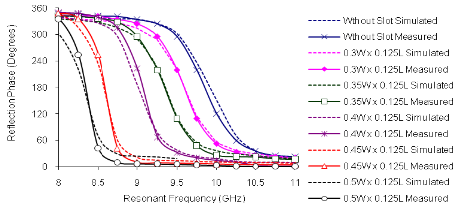
Figure 5. Simulated and measured reflection phase for different widths of rectangular slots
