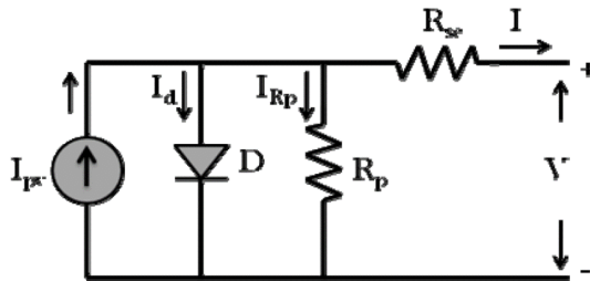
Figure 2. Solar Panel Equivalent Circuit with Parallel Resistor [15]
