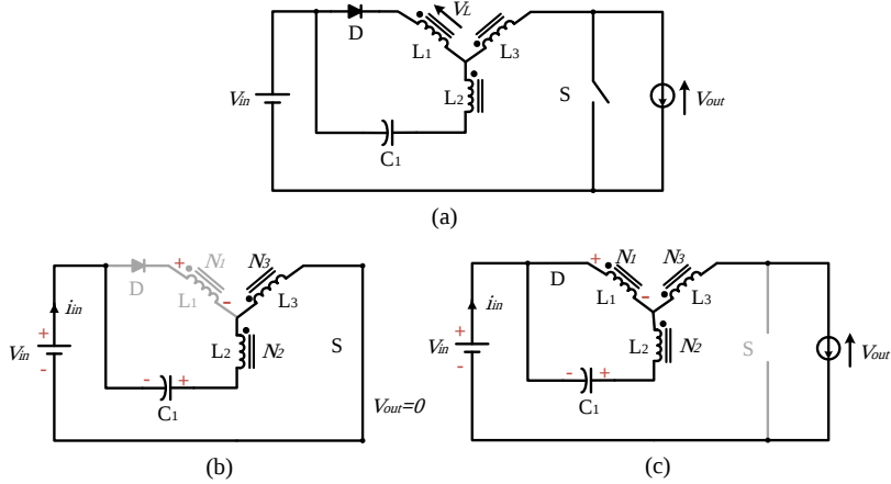
Figure 3. The quasi-Y-source impedance network and its equivalent circuit in (b) the shoot-through state and (c) the non-shoot-through state
