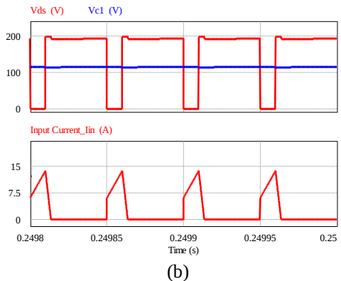
Figure 9. Steady state respond for (a) Y-source boost dc-dc converter and (b) quasi-Y-source boost dc-dc converter.
