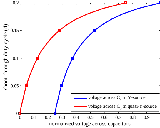
Figure 4. Comparison between normalized capacitors voltage stress.
