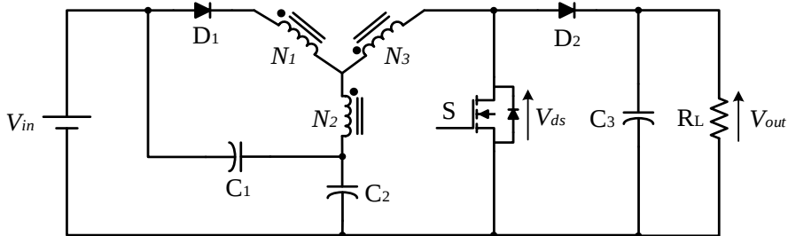
Figure 7. The improved Y-source boost dc-dc converter
