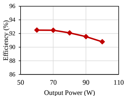
Figure 15. Measured efficiency of the proposed converter.
