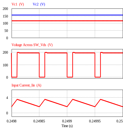
Figure 10. Simulation results for the improved Y-source boost dc-dc converter in steady state.
