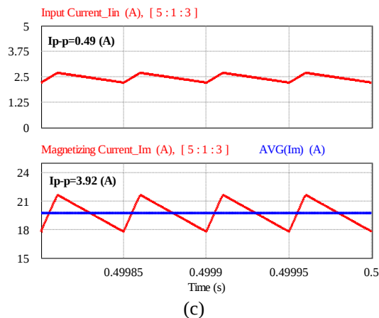
Figure 11. Input and magnetizing currents for different combination of windings turns and K=4 .
