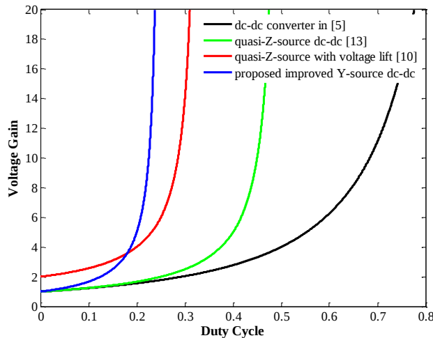
Figure 8. Comparison between voltage gain of the proposed converter and other converters
