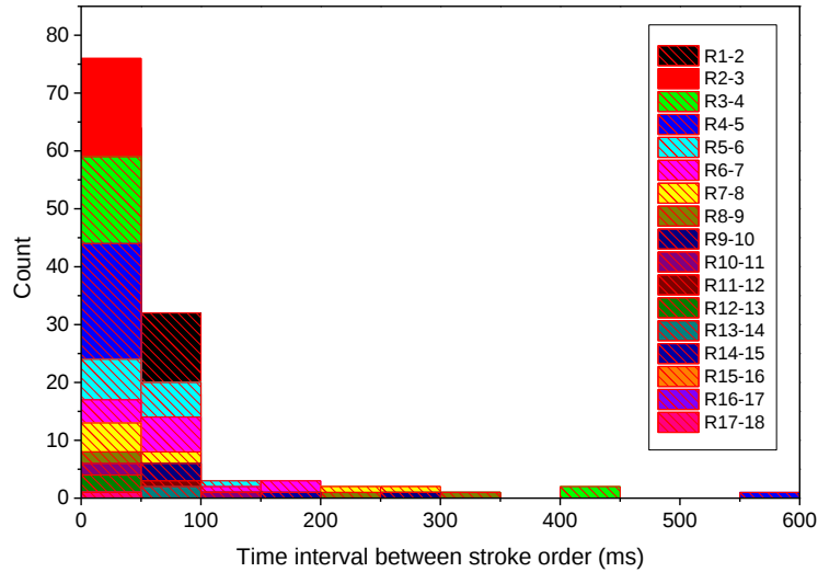
Figure 10. Histogram of return stroke order interstroke interval
