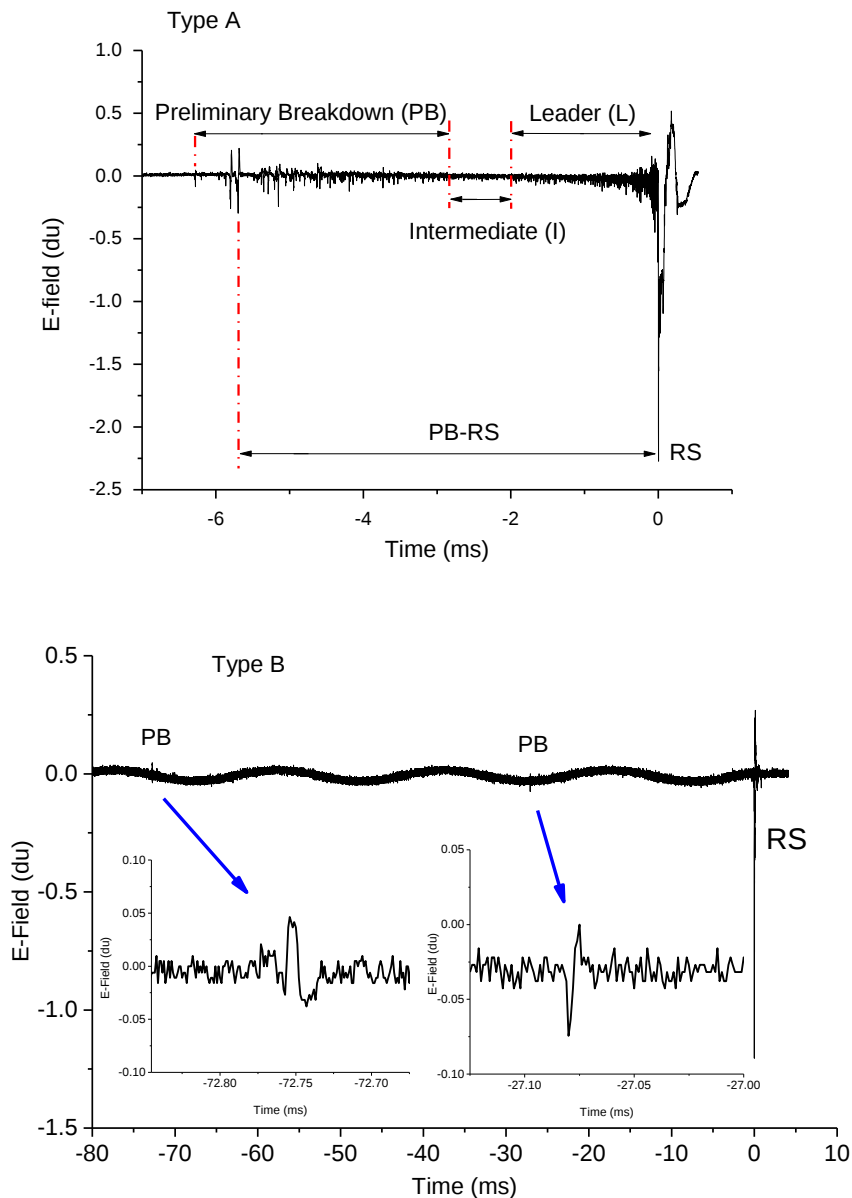
Figure 2. Typical electric field waveform of preliminary breakdown pulses for type A and B.
