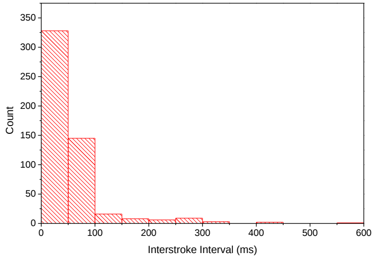
Figure 9. Histogram of interstroke interval of multiple stroke in negative lightning flashes
