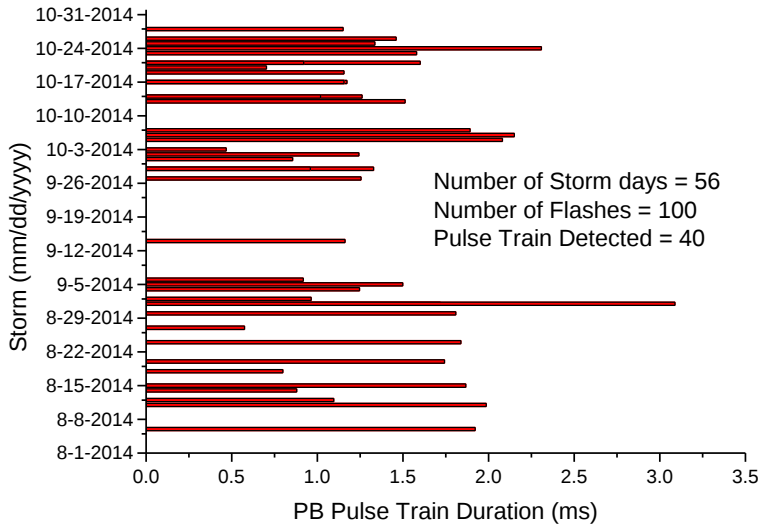
Figure 4. Histogram of PBP train duration
