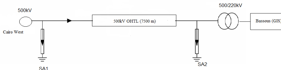
Figure 1. Single line diagram of Bassous-Cairo West power line
