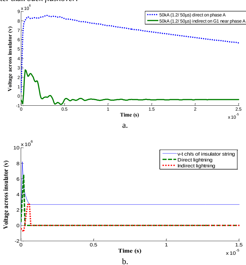
Figure 15. Voltage across phase A insulator string comparison at direct and indirect lightning strokes (a) Without using flashover model (b) With using flashover model
