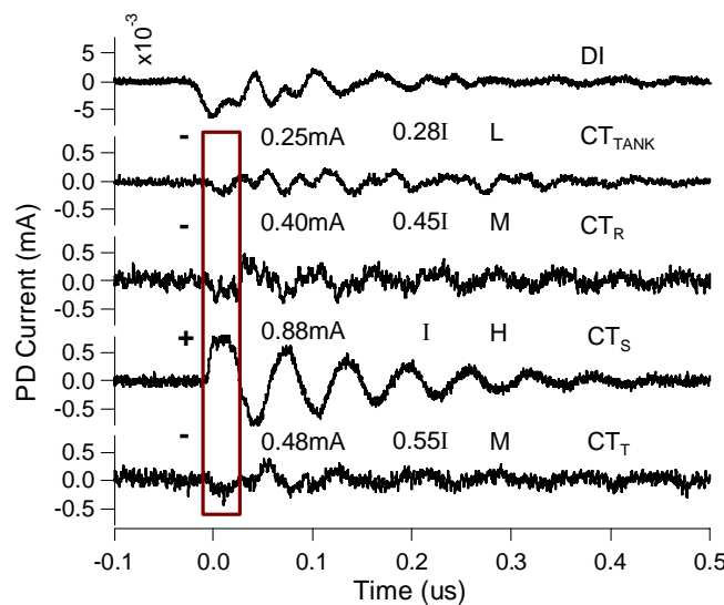
Figure 10. PD Current waveform measured for S90 particle
