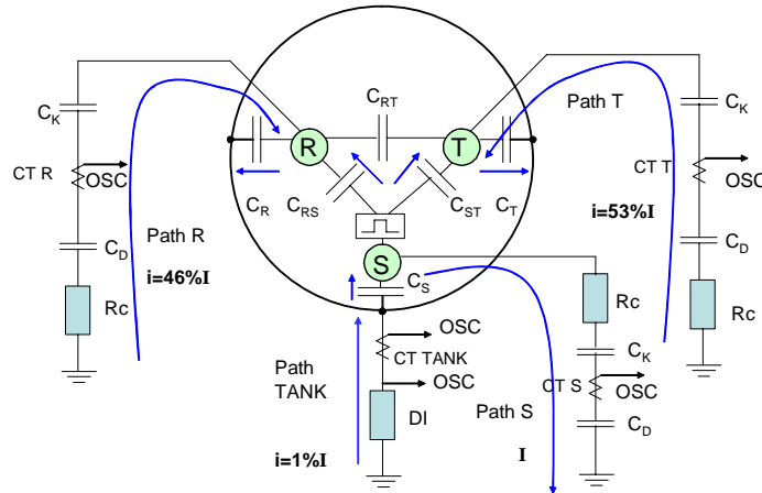
Figure 14. Equivalent circuit and path of PD current of S90 particle
