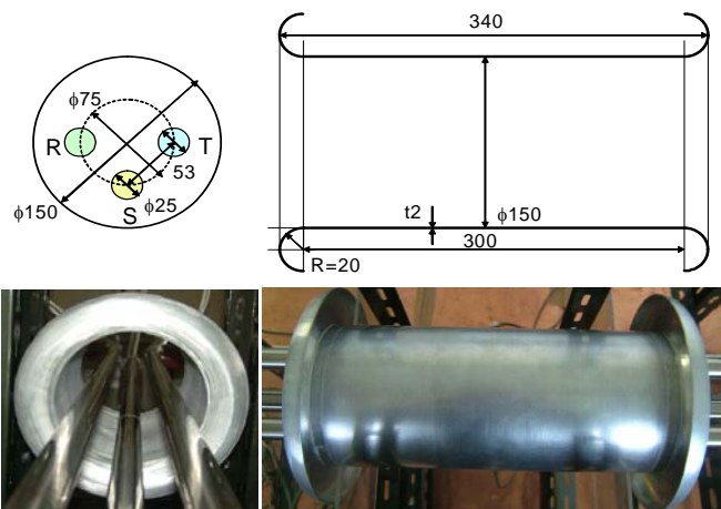
Figure 1. Layout of simplified model of three-phase GIS
